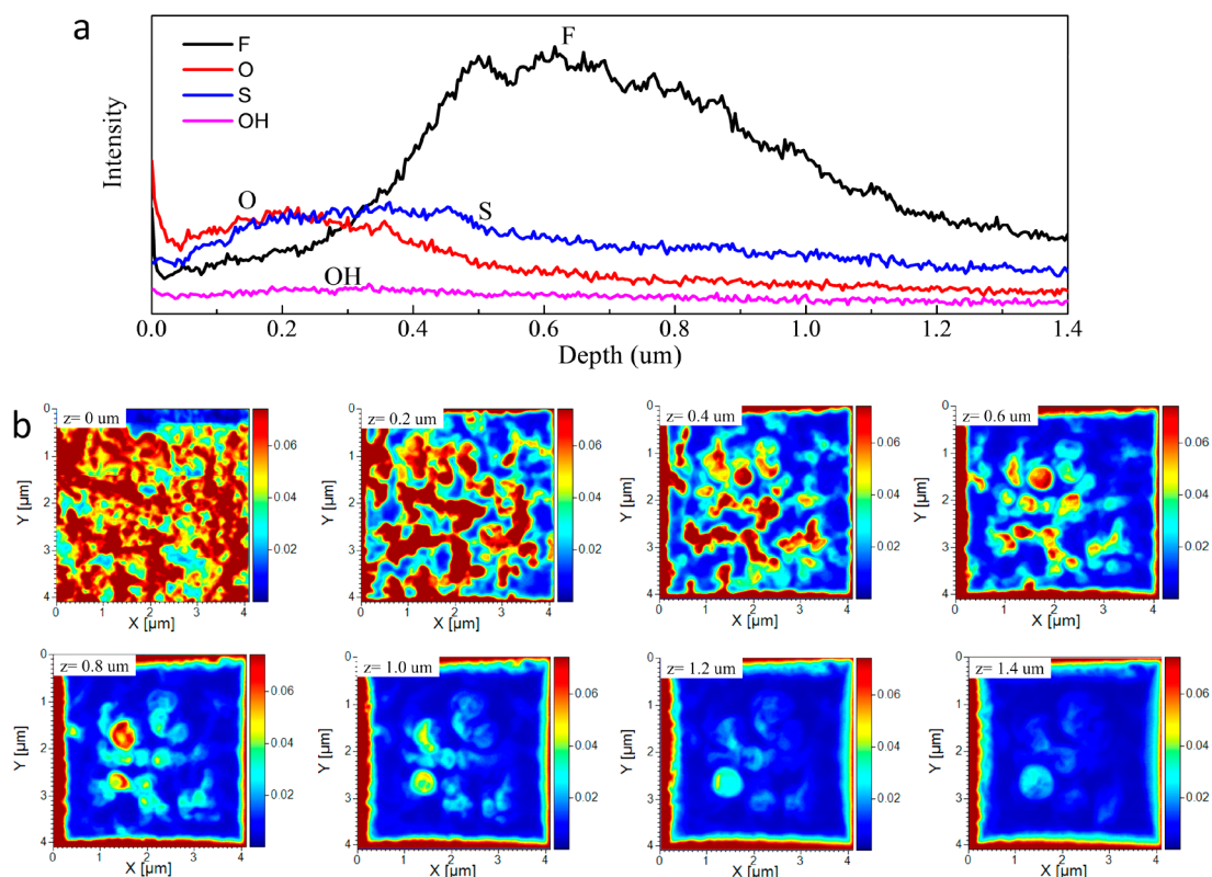
Figure 2. Time-of-flight secondary ion mass spectrometry (TOF-SIMS) analysis of cyclized \text{Mo}_6\text{S}_8 electrode after being cyclized for 40 times at 0.5 C (Negative mode). (a) TOF-SIMS depth-profiles of various chemical species, and (b) the variation of SIMS total intensity with the etching depth.
