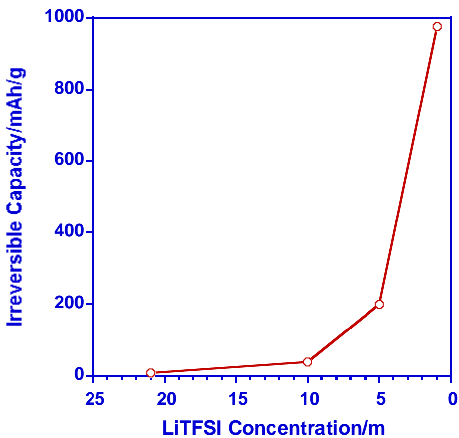
Figure S1 The irreversible capacities of full cell (LiMnO/ Mo 6 S 8 ) at various Li salt concentrations (LiTFSI-H 2 O). (a) 1 m, (b) 5 m, (c) 10 m and (d) 21.
