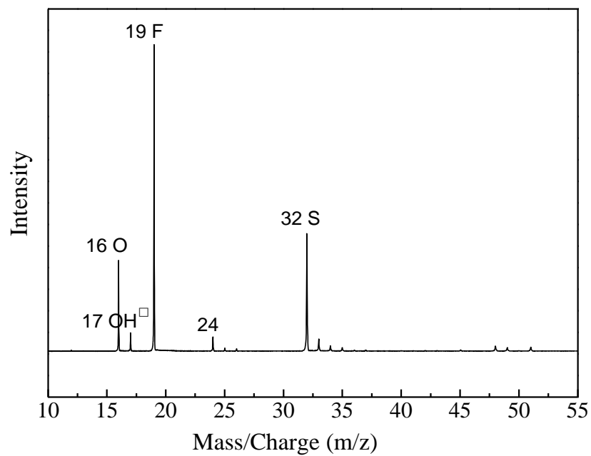
Figure S3. ToF-SIMS (Negative mode) of cycled Mo 6 S 8 electrode
