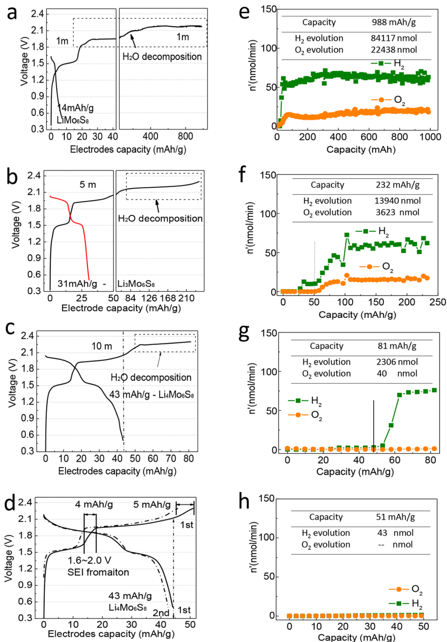
Figure 1. (a–d) Voltage profiles for the first charge–discharge profiles of full Li-ion cells constructed with \text{Mo}_6\text{S}_8 anode and \text{LiMn}_2\text{O}_4 cathode and cycled in four aqueous electrolytes of different salt concentrations. In these full cell configurations the anode and cathode are coupled at \text{LiMn}_2\text{O}_4/\text{Mo}_6\text{S}_8 = 2:1 by weight. (e–h) \text{H}_2 and \text{O}_2 evolution monitored during the first charging process using differential electrochemical mass spectrometry (DEMS) in these same aqueous full Li-ion cells.
