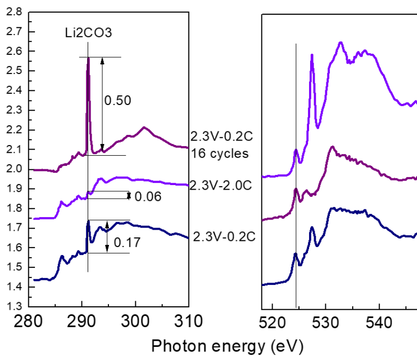
Figure S5 C and O K-edge sXAS spectra of the SEI layers formed on Mo 6 S 8 at different cycle times (1 and 16 cycles) and rates (0.2C and 2C) in bulk-sensitive TFY mode with the detected penetration depth of 100 ~ 200 nm
