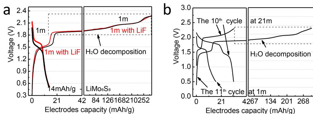
Figure 5. Solubility of aqueous SEI and the related electrochemical performance of aqueous Li-ion LiMn 2 O 4 /Mo 6 S 8 full cell: (a) in 1 m LiTFSI/H 2 O with or without being saturated with LiF; (b) the same cell in 1 m LiTFSI/H 2 O after an SEI was performed in WiSE (21 m) for 10 cycles.
