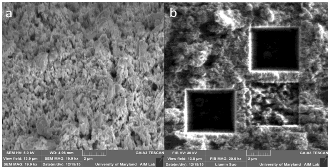
Figure S2. SEM images of cycled Mo 6 S 8 electrode. a. before FIB and b. after FIB.
