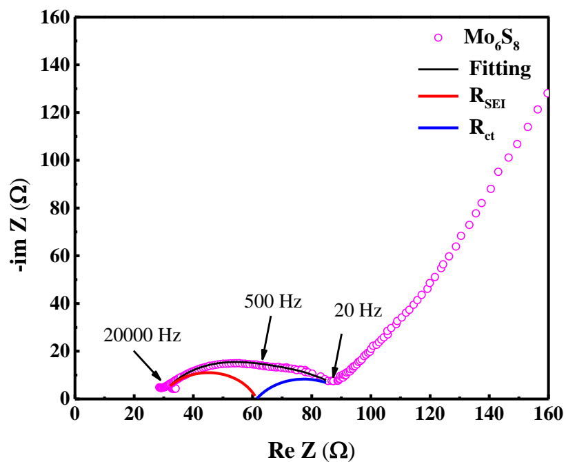
Figure. S6. Electrochemical Impedance Spectrum (EIS) of \text{Mo}_6\text{S}_8 anode after 2 cycles in three-electrode devices (Work electrode: \text{Mo}_6\text{S}_8 , Reference electrode: Ag/AgCl reference, Counter electrode: Pt electrode).
