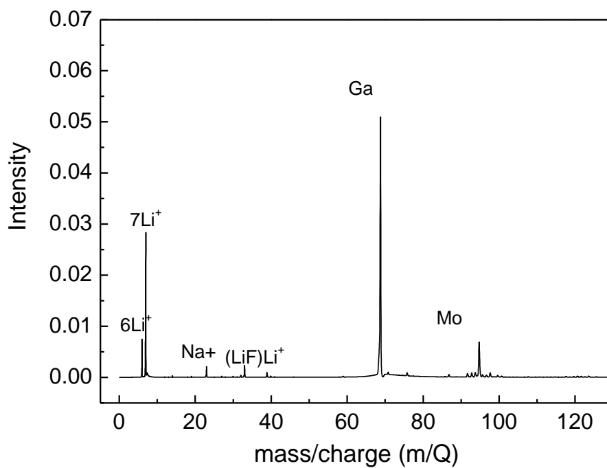
Figure S4. ToF-SIMS (Positive mode) of cycled Mo 6 S 8 electrode
