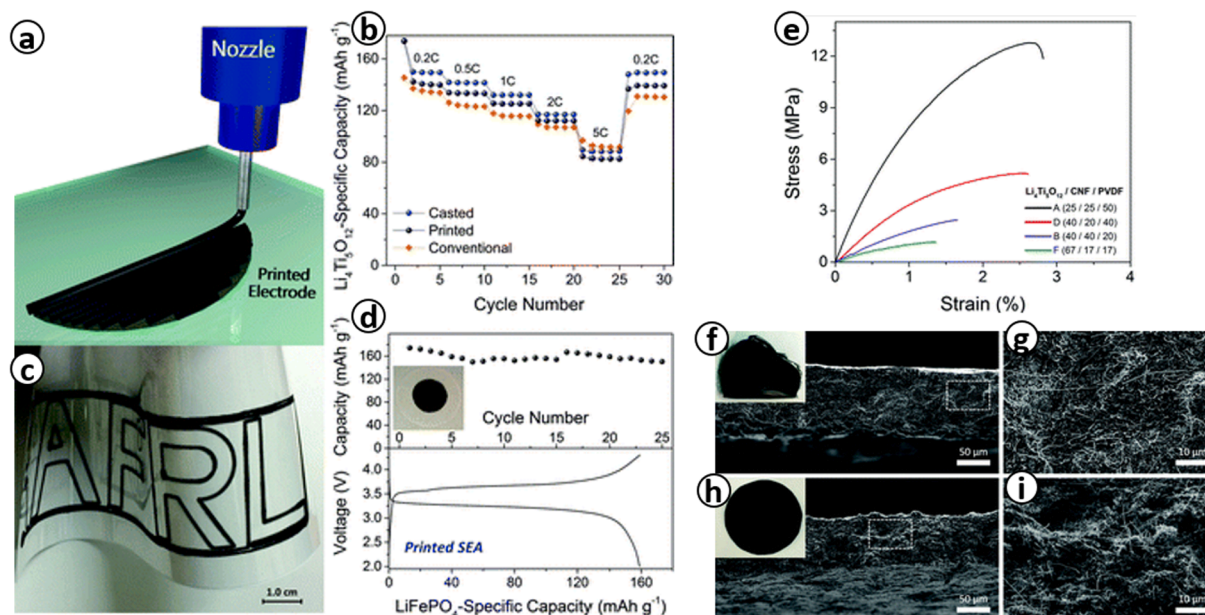
Fig. 2. Direct ink writing printing of lithium ion battery electrode. (a) Printing of active/CNF/PVDF composite electrodes at a mass ratio of 40:40:20. (b) Rate performance of printed, casted composite and a conventional \text{Li}_4\text{Ti}_5\text{O}_{12} electrode on copper under active loading between 3.0 and 3.5 \text{mg}/\text{cm}^2 . (c) Photograph of a complex filamentary printed design. (d) Cycle performance and charge/discharge profile with a photograph (inset) of a fully printed separator electrode assembly. (e) Representative uniaxial tensile stress–strain curves of \text{Li}_4\text{Ti}_5\text{O}_{12} /CNF/PVDF composites with four different mass ratios. (f–g) Photograph and cross-sectional scanning electron microscopy (SEM) images of the composite with mass ratio of 25:25:50. (h–i) Photograph and cross-sectional SEM images of the composite with mass ratio of 40:40:20 [78].
