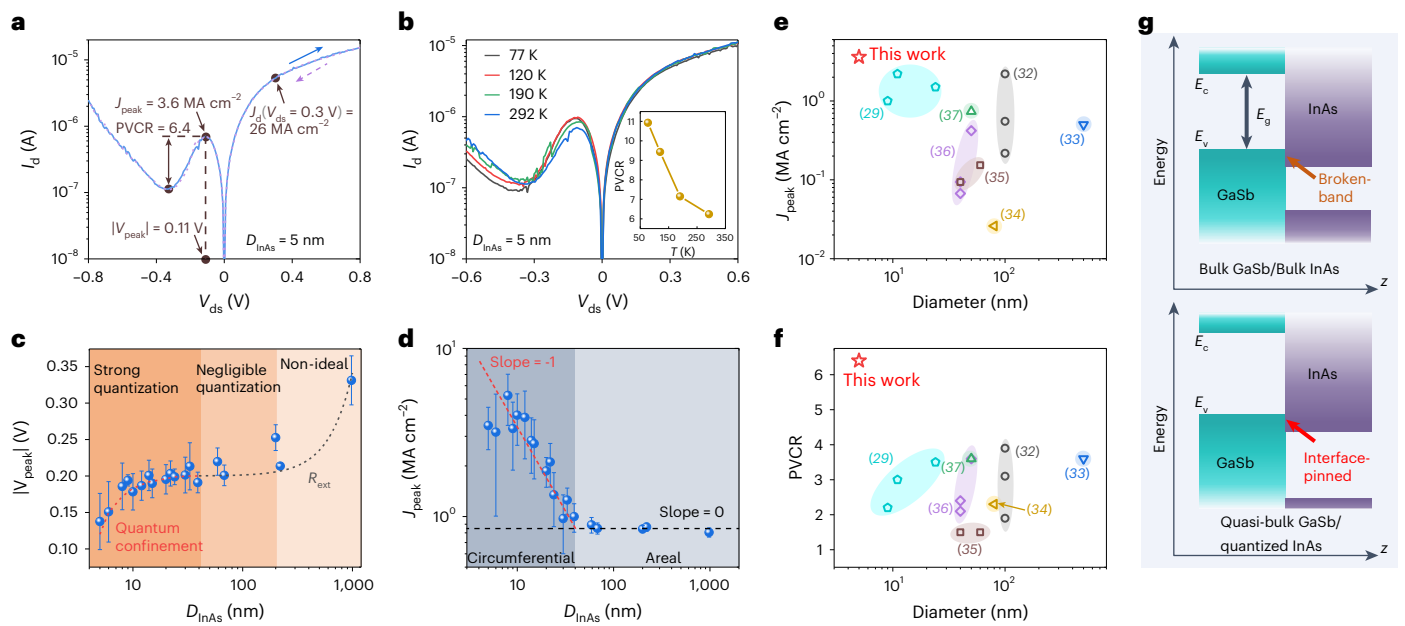
Fig. 2 | Electrical characteristics and benchmarking of vertical-nanowire Esaki diodes.
