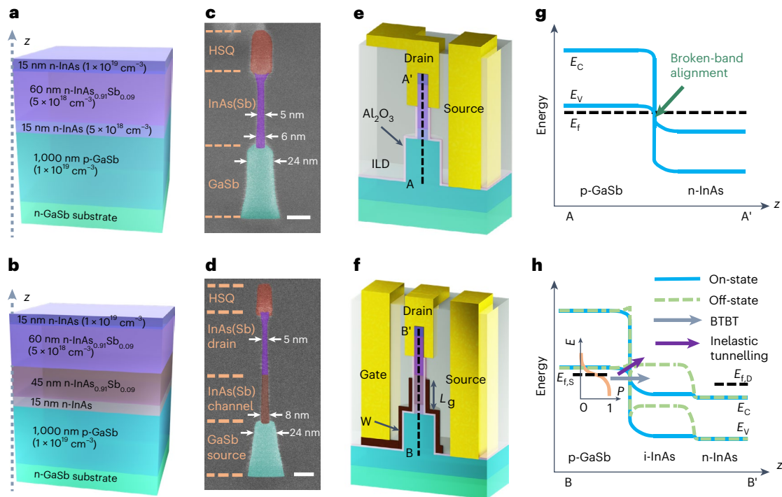
Fig. 1 | Ultra-scaled vertical-nanowire device design. a, b, Heterostructures in the fabrication of a heterojunction Esaki diode (a) and a tunnelling transistor (b). c, d, False-coloured 30°-tilted SEM images of vertical nanowires in the Esaki diode (c) and the tunnelling transistor (d), which were fabricated by dry-etching and citric acid:H 2 O 2 wet-etching with D_{\text{InAs}} of around 6 and 8 nm at the tunnelling junction, respectively. e, f, Schematics of the finished device structures for the vertical-nanowire Esaki diode (e) and vertical-nanowire tunnelling transistor (f).
