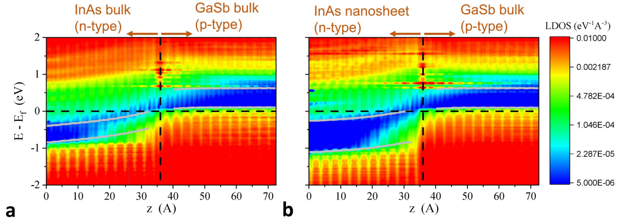
Supplementary Fig. 9 | Coupled DFT-NEGF calculations. a,b , Calculated projected local density of states (PLDOS) of the bulk GaSb/bulk InAs structure ( a ) and the bulk GaSb/confined InAs structure ( b ). Extracted band edges are labeled in ivory. A broken-band alignment at the interface could be obtained with a p- (n-) doping in GaSb (InAs).
