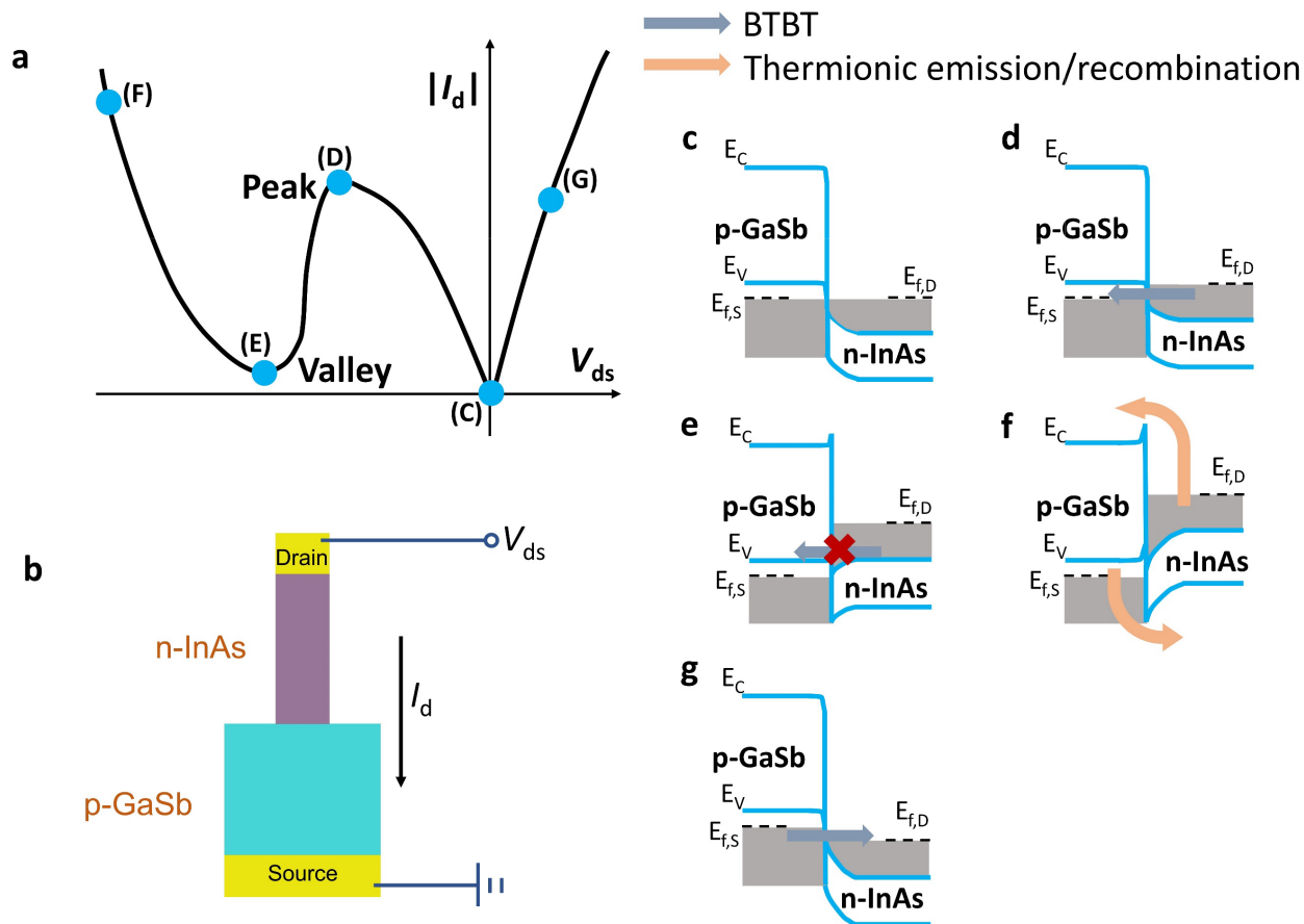
Supplementary Fig. 3 | Working principle of broken-band GaSb/InAs Esaki diode. a , Schematic I - V curve of a GaSb/InAs Esaki diode with peak and valley labeled. b , Schematic Esaki diode structure, as well as the definition of voltage and current. c-g , Schematic energy band diagrams at different bias, including thermal equilibrium ( c ), peak position ( d ), valley position ( e ), thermal current ( f ), and positive V_{ds} regimes with dominant BTBT ( g ). When a negative V_{ds} is applied, as the absolute bias value increases, peak current ( I_{peak} ) due to BTBT of electrons from InAs to GaSb is reached ( d ), followed by an NDR region with a valley current ( I_{valley} ) ( e ). Finally, the current increases again due to thermionic emission ( f ). When a positive V_{ds} is applied, the BTBT current of electrons from GaSb to InAs keeps increasing as the bias increases ( g ). This is the working regime for tunneling transistors.
