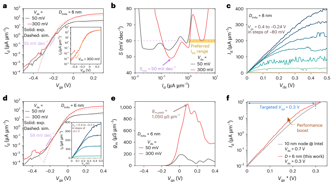
Fig. 3 | Electrical characteristics of ultra-scaled vertical-nanowire tunnelling transistors. a–c, Transfer characteristics (a), subthreshold swing ( S ) versus I_d (b) and output characteristics (c) of a transistor with D_{\text{InAs}} = 8 nm. Inset in a, Hysteresis sweep. S_{\text{min}} denotes the minimum S , and I_{60} denotes the maximum I_d for sub-60 \text{mV dec}^{-1} operation. d–f, Transfer characteristics (d), transconductance ( g_m ) characteristics (e) and performance comparison with CMOS technology at the 10 nm node 43 (f) of a transistor with D_{\text{InAs}} = 6 nm. g_{m,\text{peak}}
