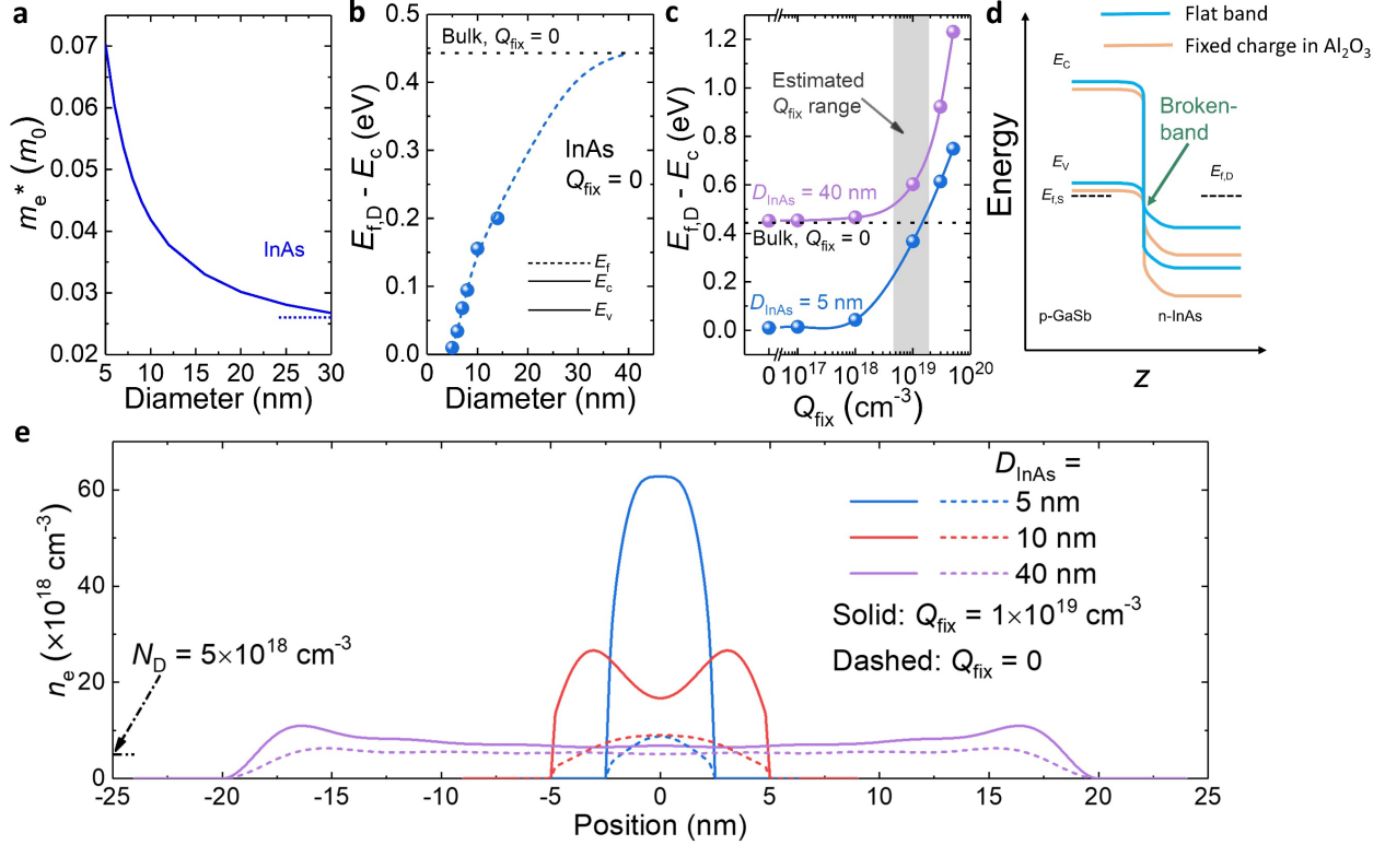
Supplementary Fig. 5 | Two-dimensional simulations of nanowire cross-sections and resulting band diagrams. a , Electron effective mass ( m_e^* ) for InAs versus D_{\text{InAs}} . The dotted line indicates the value for the bulk material. m_0 denotes the mass of a free electron. The simulations were carried out using 8-band \mathbf{k}\cdot\mathbf{p} approach with a circular semiconductor cross-sectional area surrounded by 3-nm \text{Al}_2\text{O}_3 . b,c , Self-consistent Poisson-Schrödinger simulations using 8-band \mathbf{k}\cdot\mathbf{p} approach with a circular n-InAs ( N_D = 5 \times 10^{18} \text{ cm}^{-3} ) cross-sectional area (except for simulations with D_{\text{InAs}} = 40 nm, in which the effective-mass method was carried out with the bulk InAs electron effective mass value) surrounded by a 3-nm \text{Al}_2\text{O}_3 . In b , the position of the lowest conduction sub-band with respect to the Fermi level (i.e., E_f - E_c ) was simulated as a function of diameter (solid symbols) without fixed charge in \text{Al}_2\text{O}_3 . Due to the exponentially increasing computational burden together with convergence issues in the self-consistent 8-band \mathbf{k}\cdot\mathbf{p} simulations, we carried out simulations till a largest diameter of 14 nm. The trend line is plotted till 40 nm. The position of the conduction band edge for bulk InAs is also indicated. In c , E_f - E_c was simulated as a function of fixed charge density ( Q_{\text{fix}} ) in \text{Al}_2\text{O}_3 for D_{\text{InAs}} = 5 and 40 nm, respectively, indicating an accumulation of electrons as E_c is farther away from E_f with increasing Q_{\text{fix}} . Given that the presence of Q_{\text{fix}} has a minor influence on D_{\text{InAs}} = 40 nm devices but a significant influence on D_{\text{InAs}} = 5 nm devices, a possible Q_{\text{fix}} range is estimated. d , Schematic band diagrams for Esaki diodes with a broken-band alignment at the junction, where the influence of Q_{\text{fix}} is also shown. e , One-dimensional slice of electron concentration ( n_e ) across VNW with different D_{\text{InAs}} with and without Q_{\text{fix}} in \text{Al}_2\text{O}_3 is shown. All the simulations were performed at 300 K.
